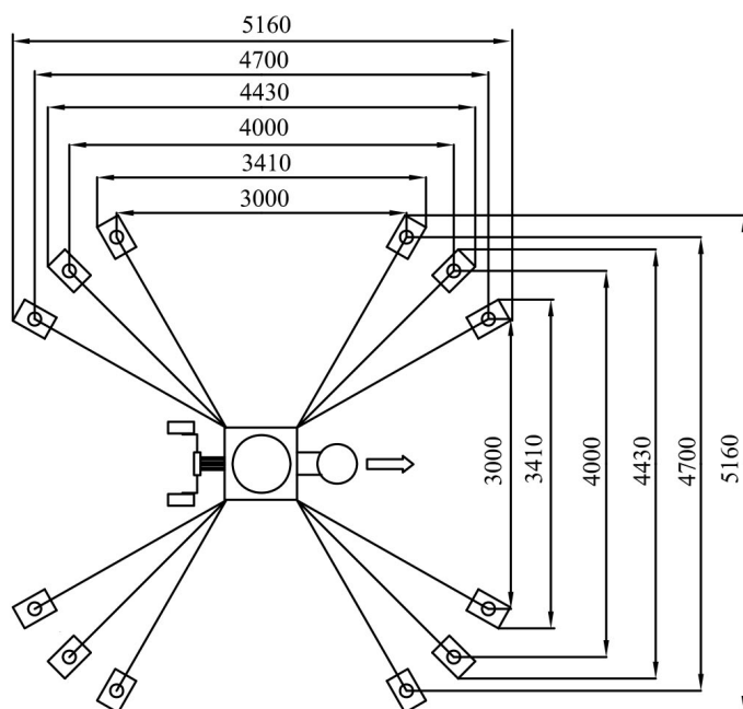
Measurement (when undercarriage is not elevated)
